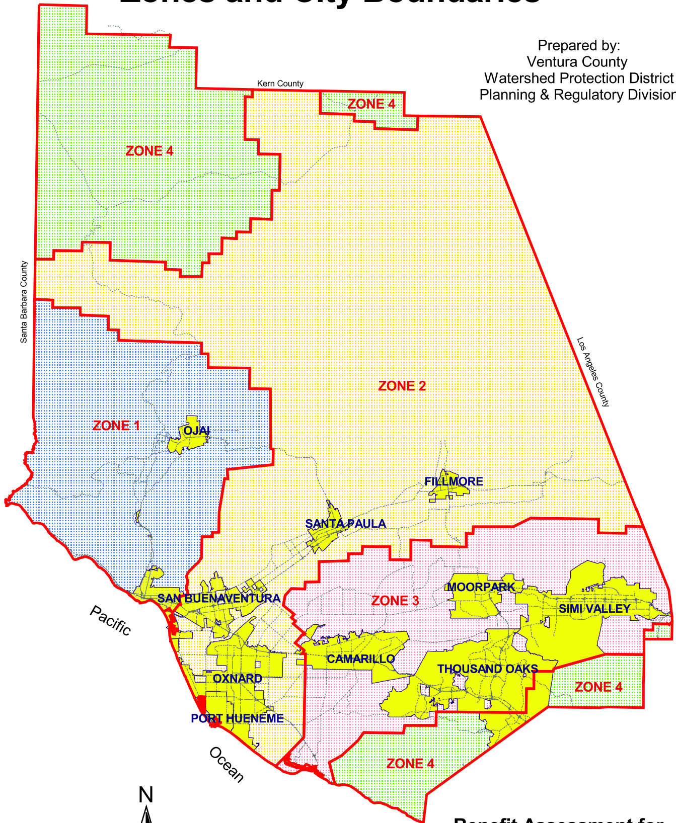
Benefit Assessment for Flood Control Fiscal Year 2017-2018 Figure 1
