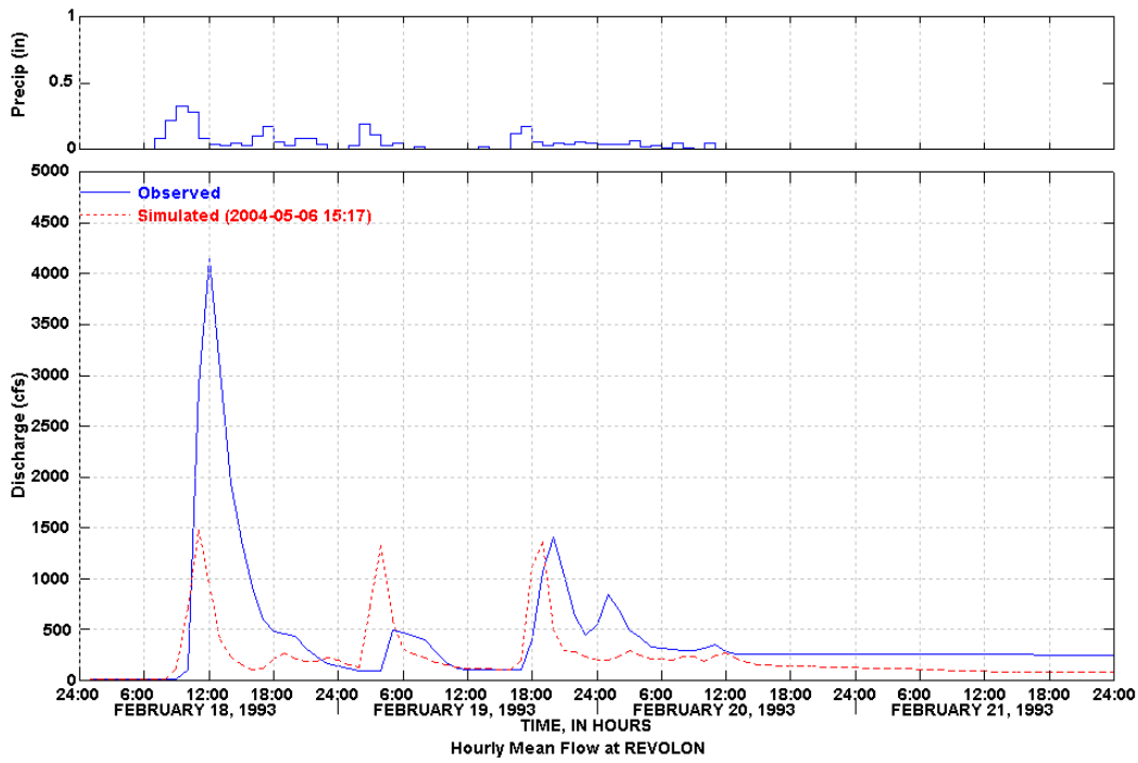
Figure 35 Simulated and Observed February 18-21, 1993 Storm Event
