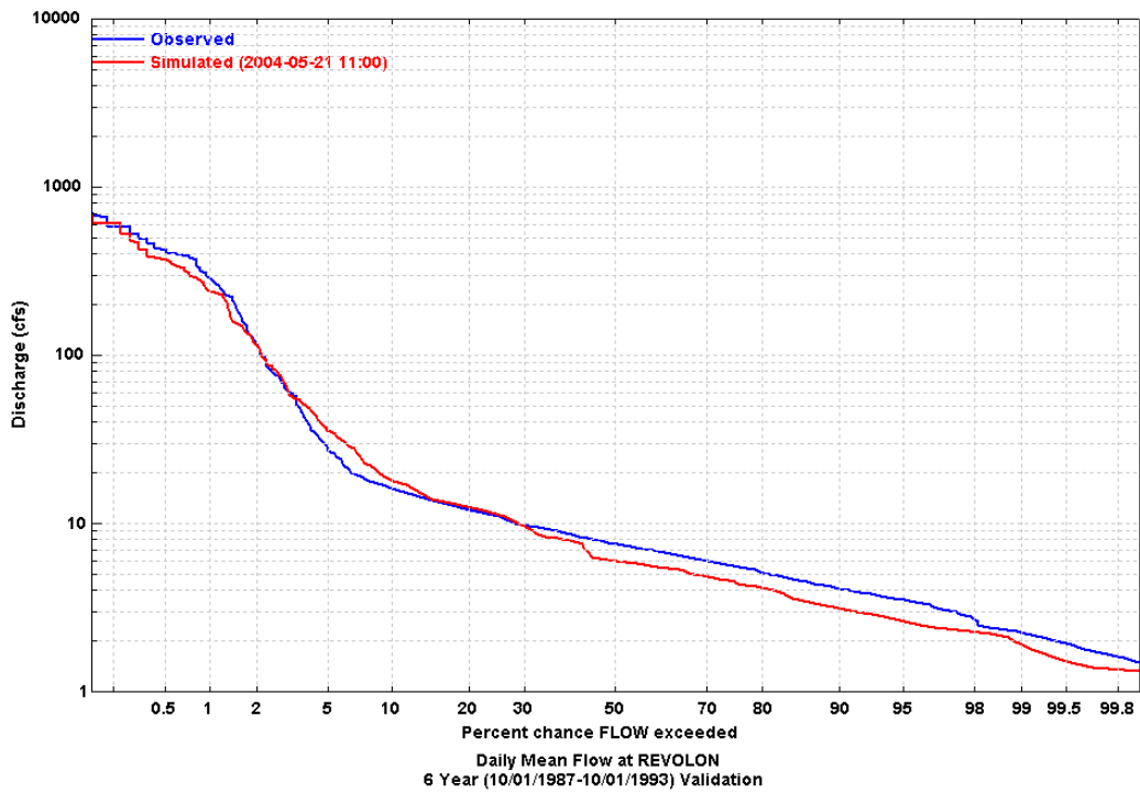
Figure 21 Simulated and Observed Daily Flow Duration Curve at Revolon
