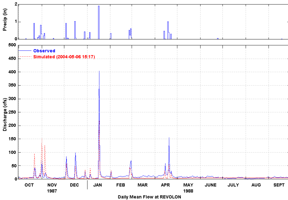
Figure 26 Simulated and Observed Daily Flow at Revolon (WY 1988)
