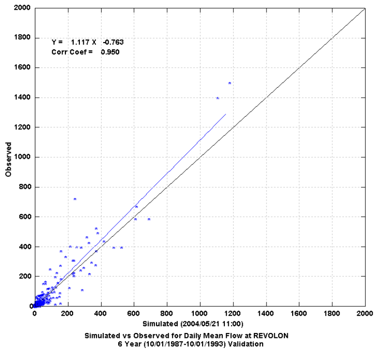
Figure 22 Daily Scatter Plot of Simulated versus Observed Flow at Revolon
