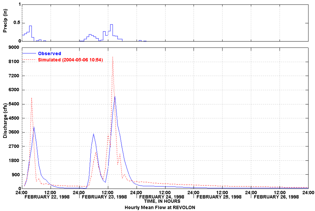
Figure 19 Simulated and Observed February 22-26, 1998 Storm Event
