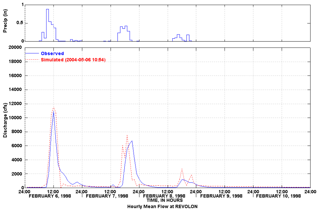
Figure 18 Simulated and Observed February 6-10, 1998 Storm Event
