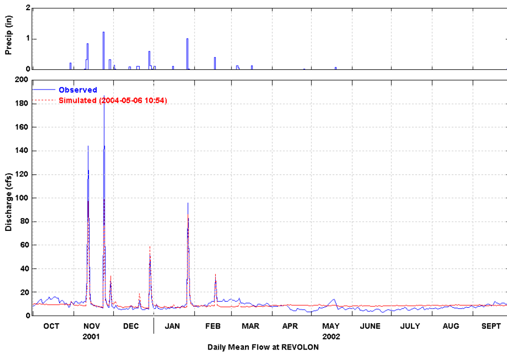
Figure 14 Simulated and Observed Daily Flow at Revolon (WY 2002)
