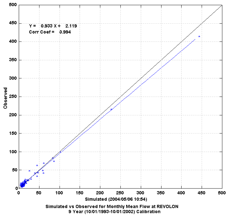
Figure 3 Monthly Scatter Plot of Simulated versus Observed Flow at Revolon
