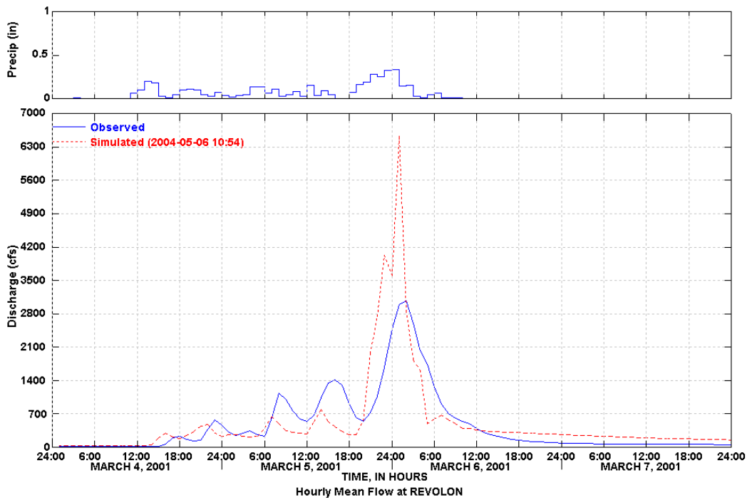
Figure 20 Simulated and Observed March 4-7, 2001 Storm Event
