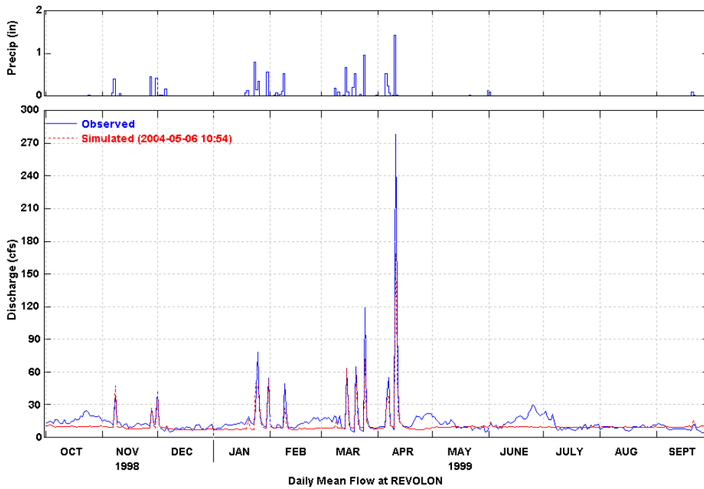
Figure 11 Simulated and Observed Daily Flow at Revolon (WY 1999)
