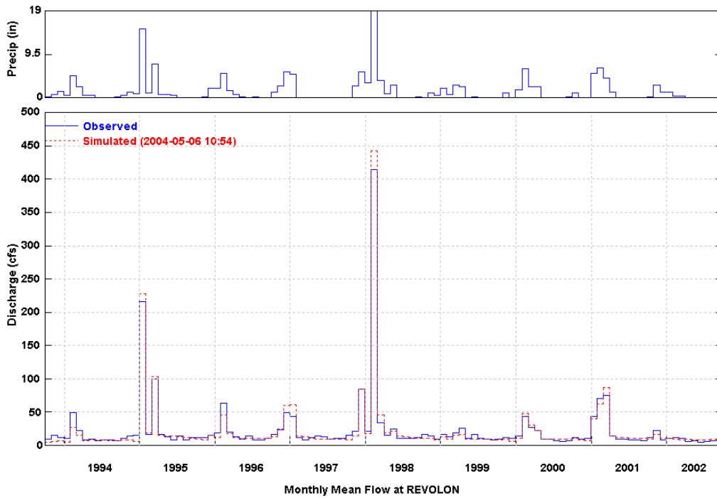
Figure 5 Simulated and Observed Monthly Flow at Revolon (WY 1994-2002)
