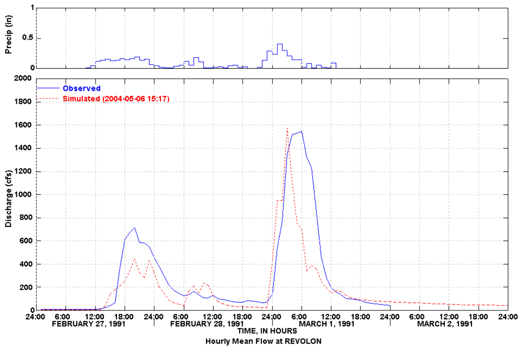
Figure 32 Simulated and Observed February 27 - March 2, 1991 Storm Event
