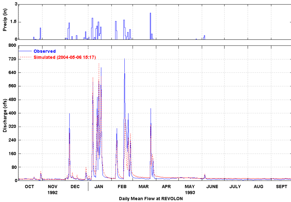
Figure 31 Simulated and Observed Daily Flow at Revolon (WY 1993)
