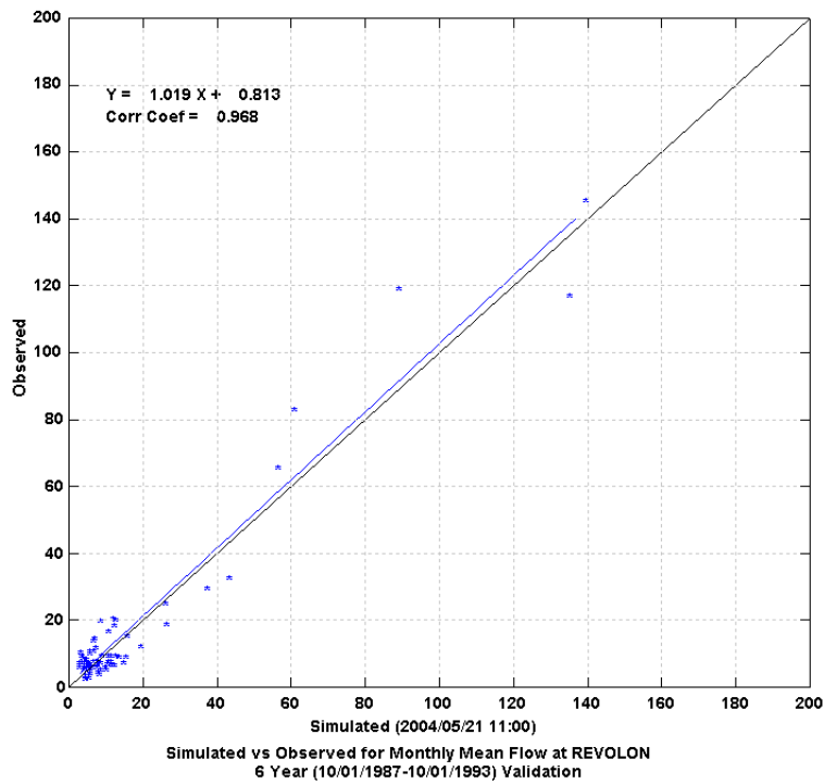
Figure 23 Monthly Scatter Plot of Simulated versus Observed Flow at Revolon
