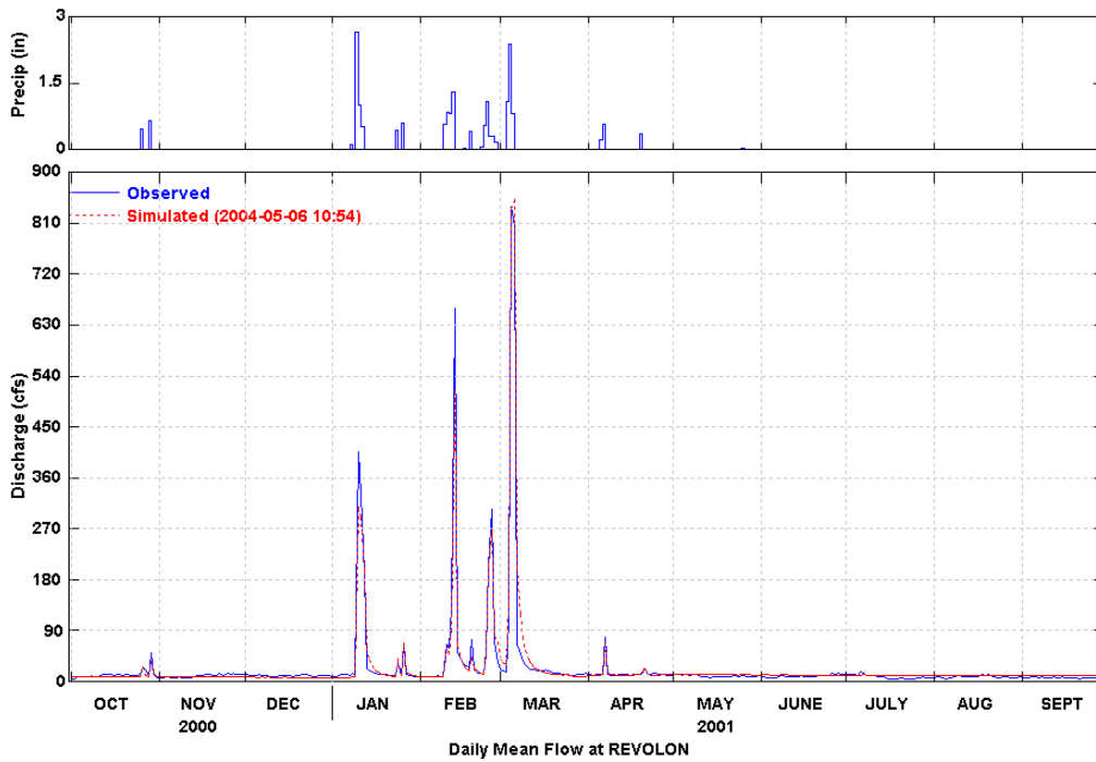
Figure 13 Simulated and Observed Daily Flow at Revolon (WY 2001)
