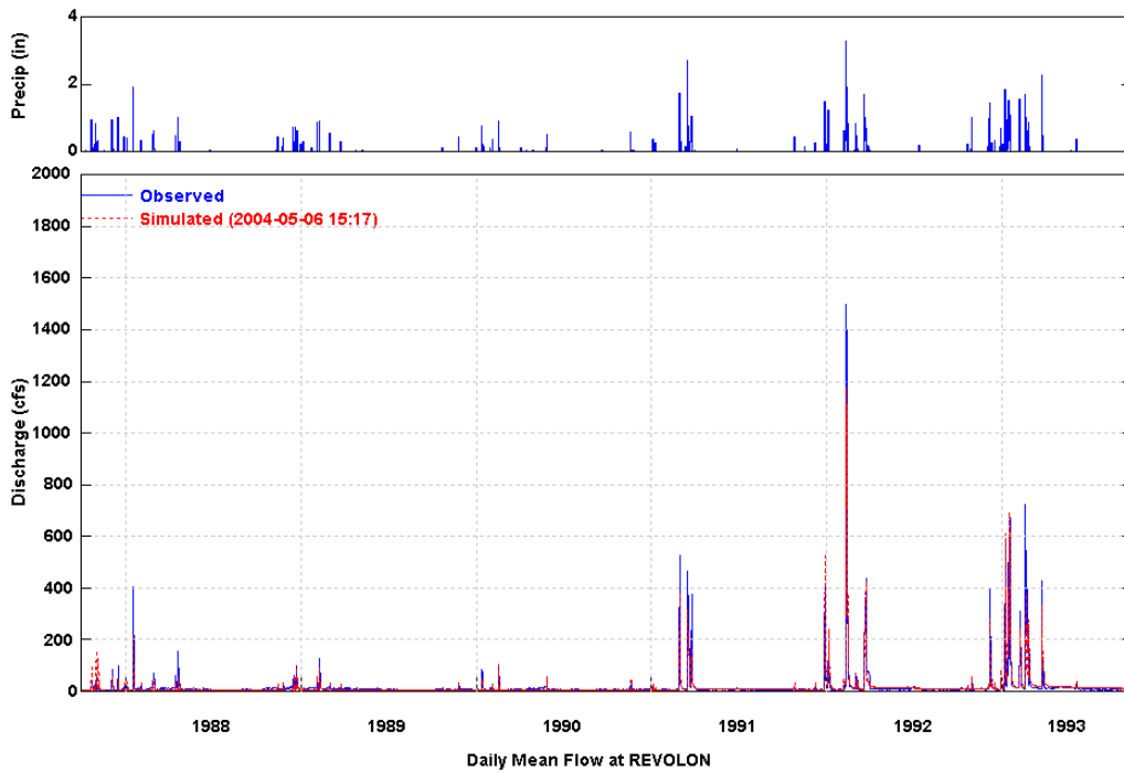
Figure 24 Simulated and Observed Daily Flow at Revolon (WY 1988-1993)
