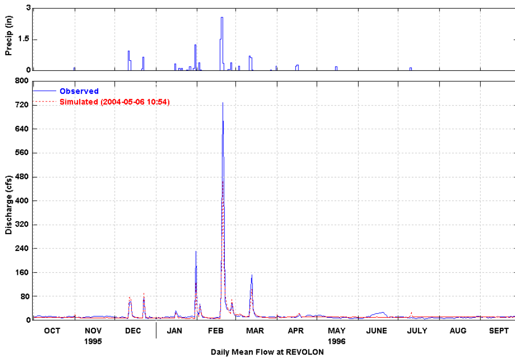
Figure 8 Simulated and Observed Daily Flow at Revolon (WY 1996)
