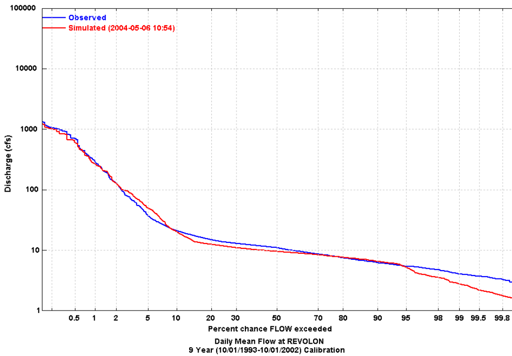
Figure 1 Simulated and Observed Daily Flow Duration Curve at Revolon
