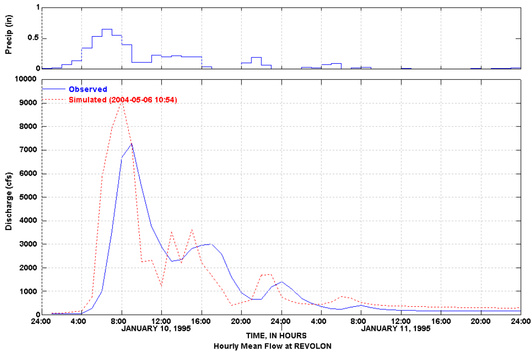
Figure 15 Simulated and Observed January 10-11, 1995 Storm Event
