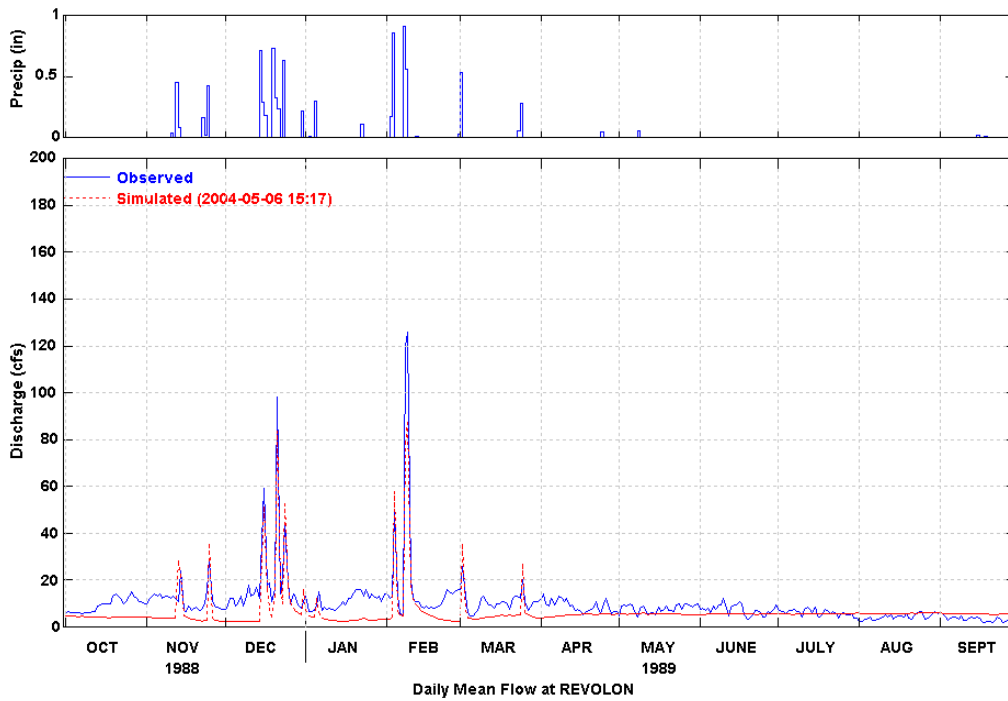
Figure 27 Simulated and Observed Daily Flow at Revolon (WY 1989)
