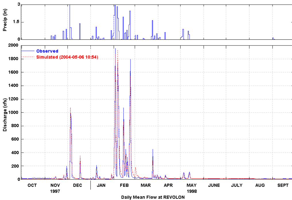
Figure 10 Simulated and Observed Daily Flow at Revolon (WY 1998)
