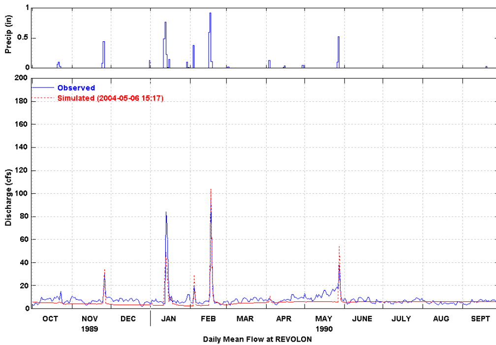
Figure 28 Simulated and Observed Daily Flow at Revolon (WY 1990)
