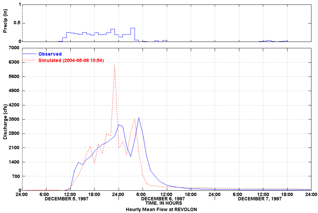
Figure 17 Simulated and Observed December 5-7, 1997 Storm Event
