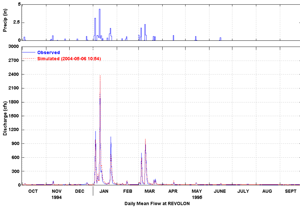
Figure 7 Simulated and Observed Daily Flow at Revolon (WY 1995)
