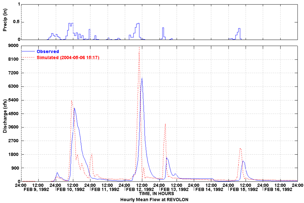
Figure 33 Simulated and Observed February 9-16, 1992 Storm Event
