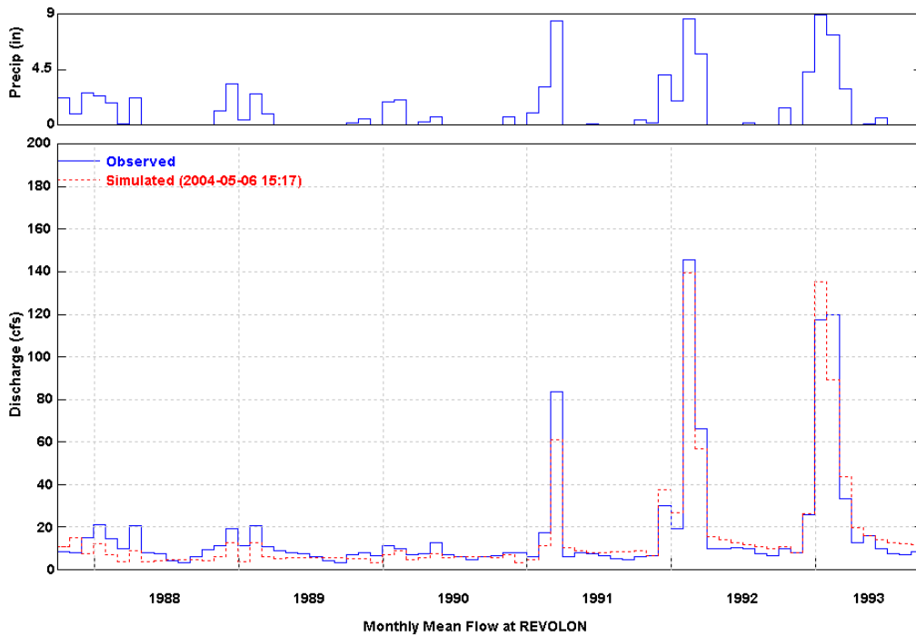
Figure 25 Simulated and Observed Monthly Flow at Revolon (WY 1988-1993)
