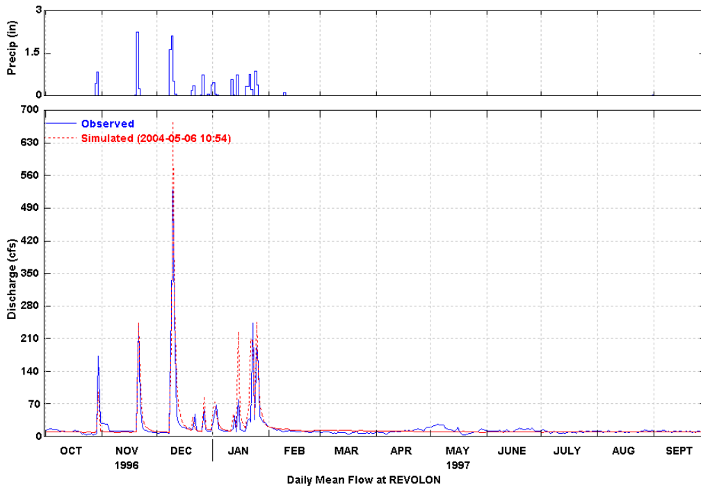
Figure 9 Simulated and Observed Daily Flow at Revolon (WY 1997)
