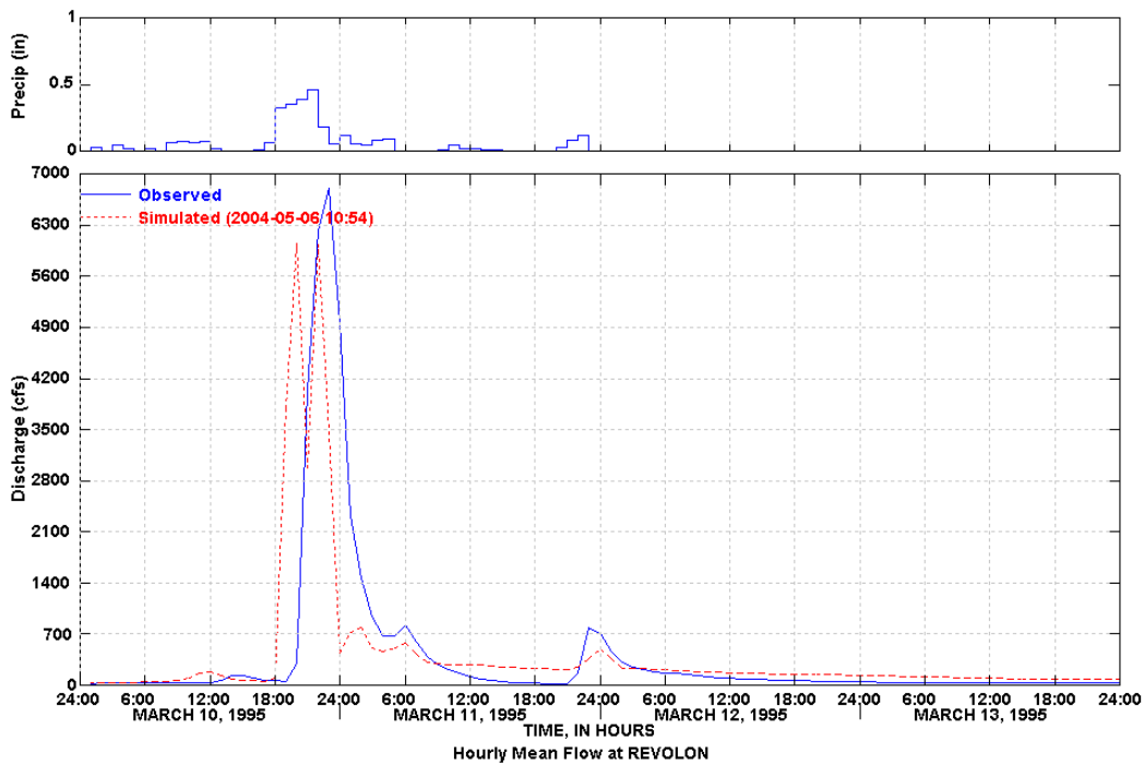
Figure 16 Simulated and Observed March 10-13, 1995 Storm Event
