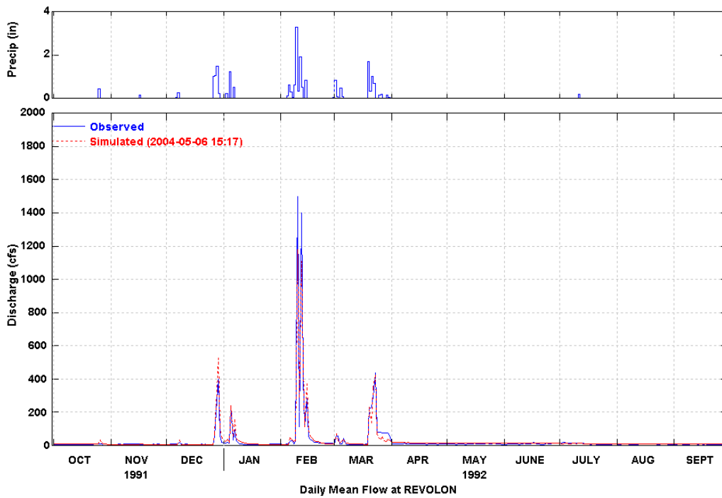
Figure 30 Simulated and Observed Daily Flow at Revolon (WY 1992)
