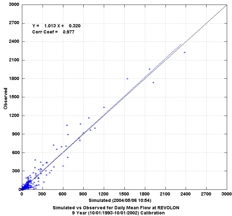
Figure 2 Daily Scatter Plot of Simulated versus Observed Flow at Revolon
