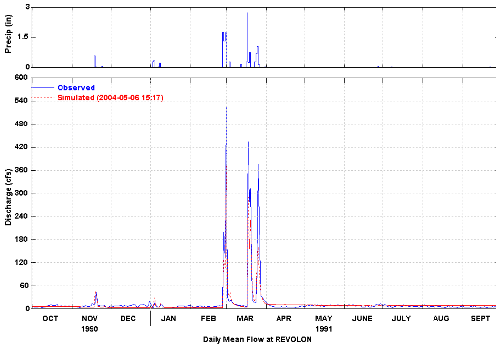
Figure 29 Simulated and Observed Daily Flow at Revolon (WY 1991)
