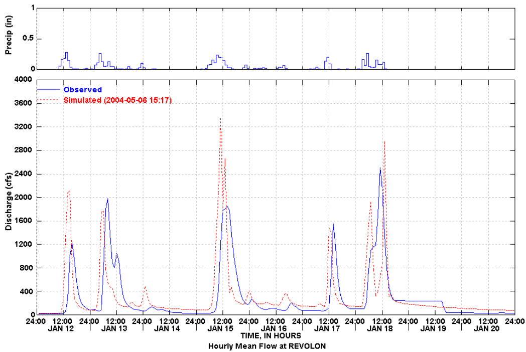
Figure 34 Simulated and Observed January 12-20, 1993 Storm Event
