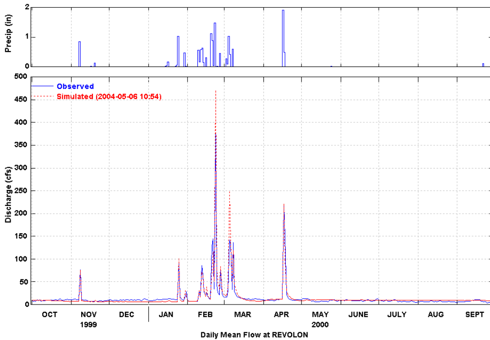
Figure 12 Simulated and Observed Daily Flow at Revolon (WY 2000)
