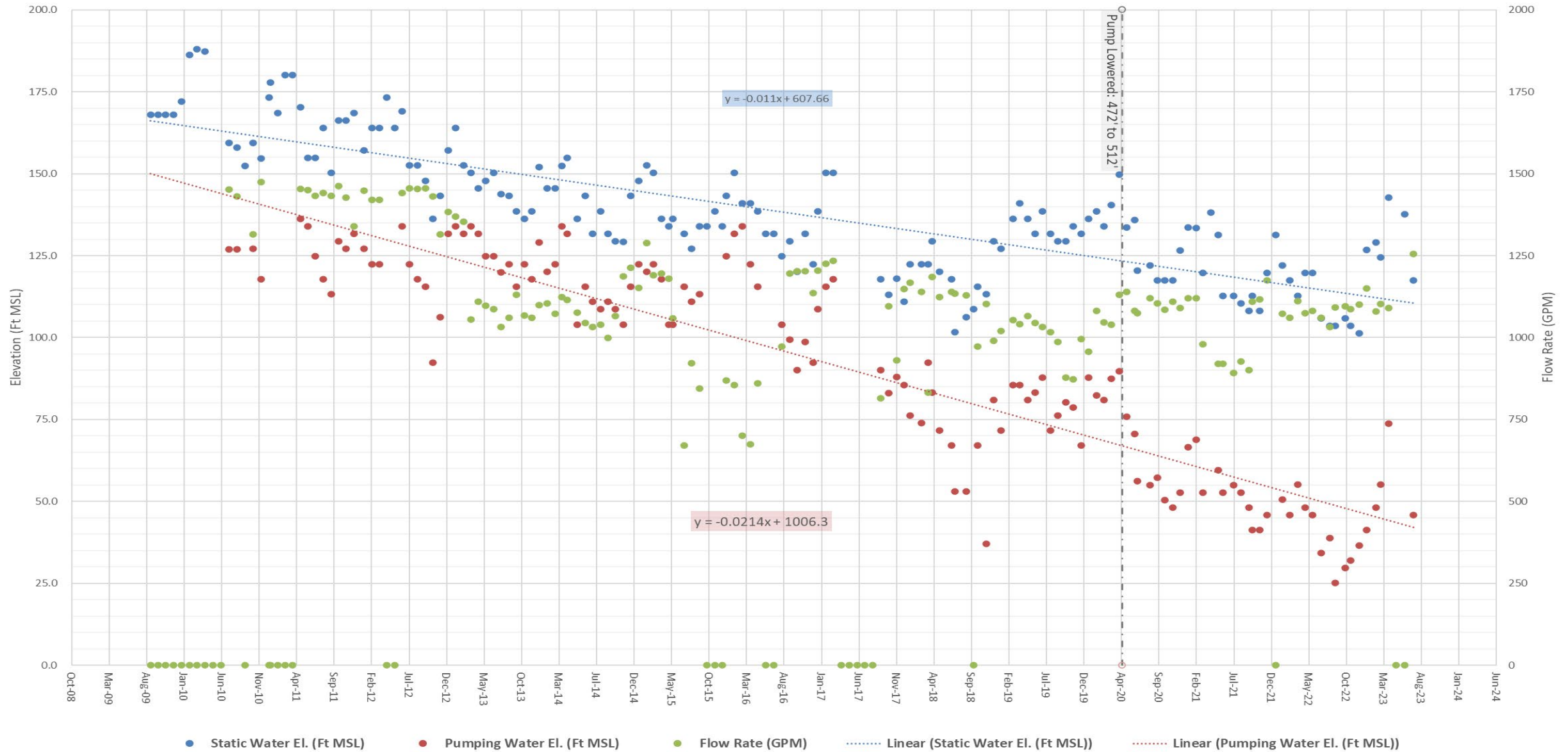
VCWWD No. 19 - Well No. 4 Hydrograph (Surface El. 512')
